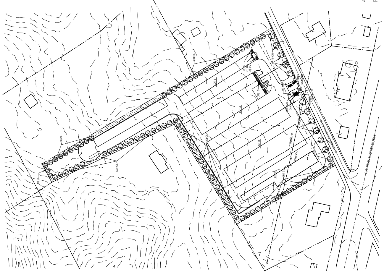
LANDSCAPE PLAN SCALE: 1"=40'
