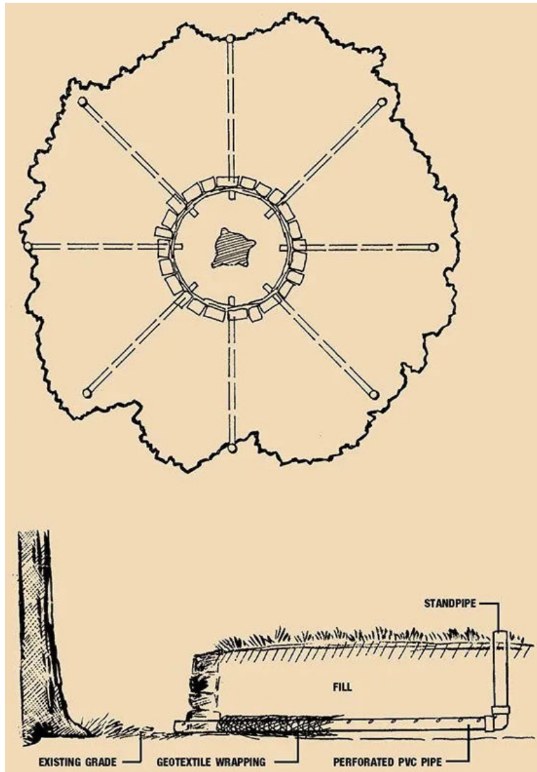
( https://extension.psu.edu/media/wysiwyg/extensions/catalog_product/93790c87d16745e5b22ccf3dd88941b9/f/i/figure22-jpg_1.jpg ) Figure 22. Aeration systems should be designed by professionals and used only when absolutely necessary. The effectiveness of aeration systems is debatable. Some of the disadvantages of 4-inch PVC pipe may be avoided by using a flexible drainage system.
