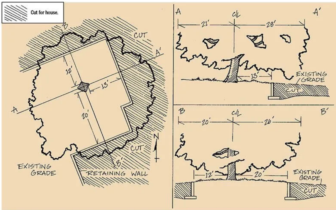
Figure 13. Information from a tree report and tree preservation plan can be used to prepare plan and elevation drawings of proposed construction impacts to trees. These drawings help developers visualize the impacts soil compaction and required limb and root pruning will have on trees.
