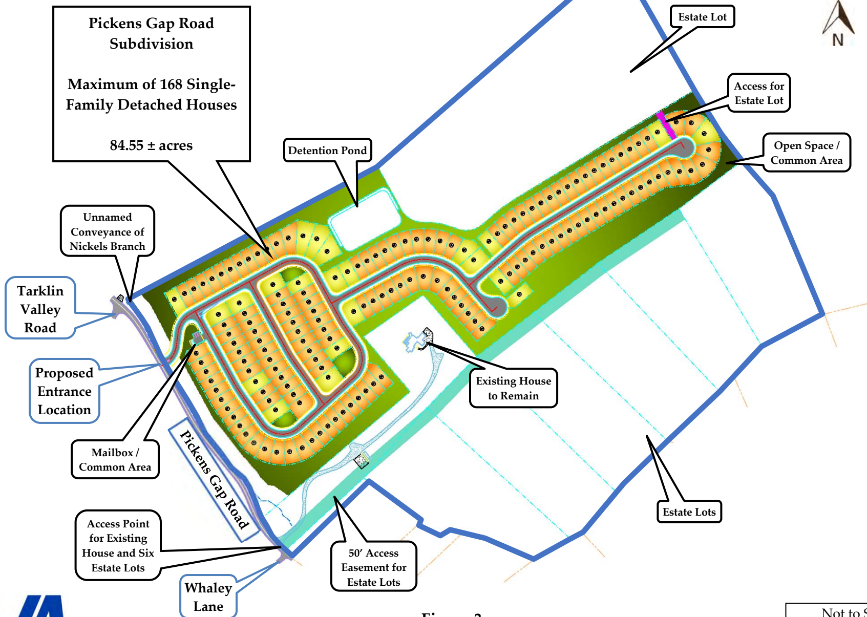
Figure 3 Proposed Plan Layout Pickens Gap Road Subdivision
